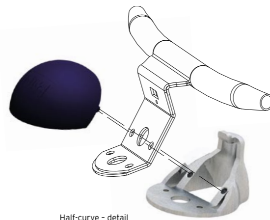
Half-curve - detail
